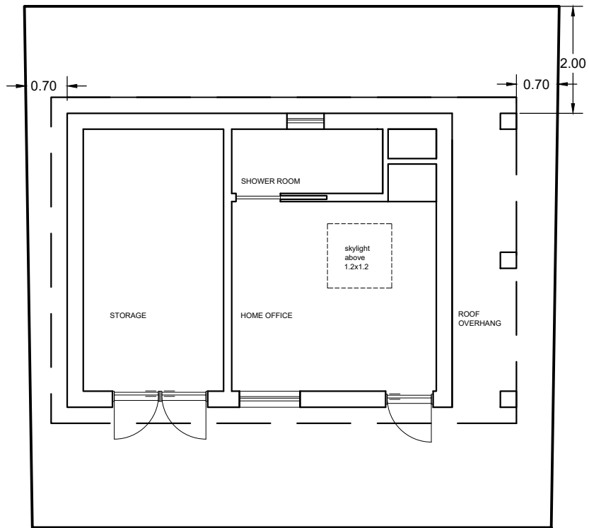
FLOOR LAYOUT Internal area: 39.6 sqm
