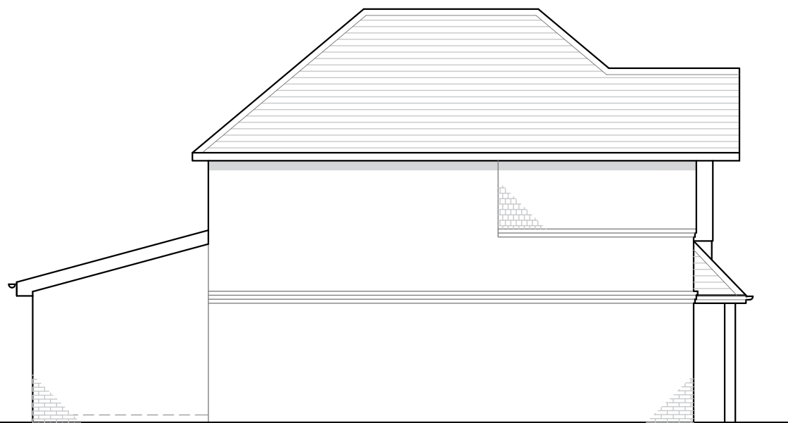
0.3 PROPOSED SIDE ELEVATION
