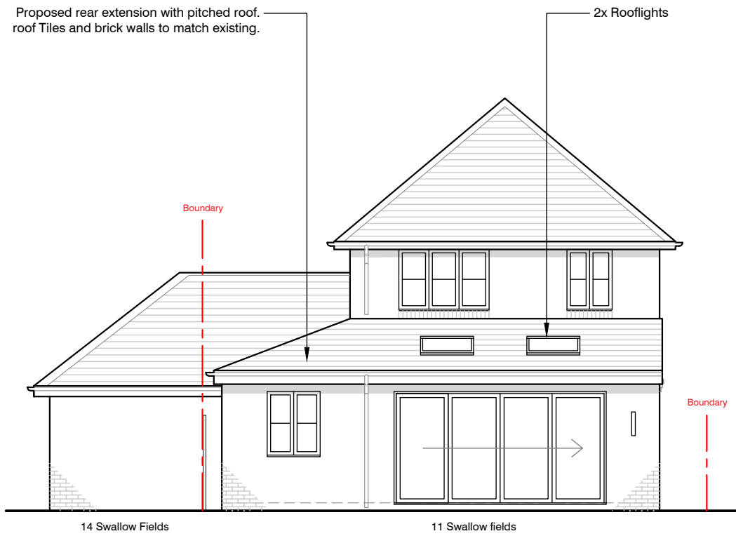
01. PROPOSED REAR ELEVATION
