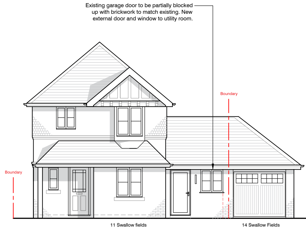
0.2 PROPOSED FRONT ELEVATION
