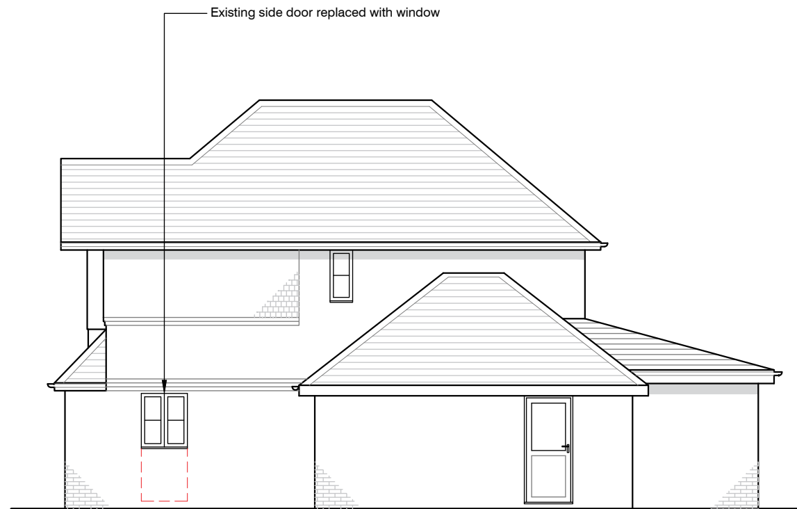
0.4 PROPOSED SIDE ELEVATION
