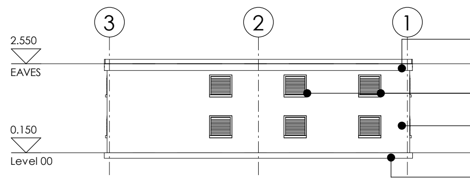
WEST ELEVATION 1 : 100
