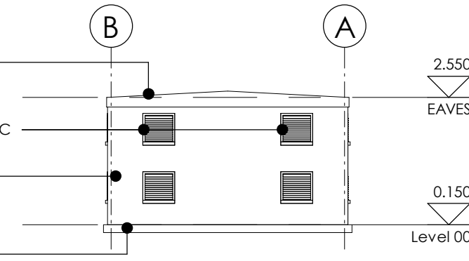
SOUTH ELEVATION 1 : 100
