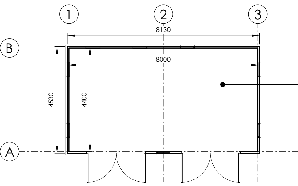
GROUND PLAN 1 : 100
