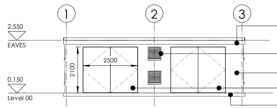
EAST ELEVATION 1 : 100
