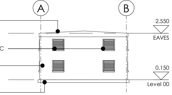
NORTH ELEVATION 1 : 100
